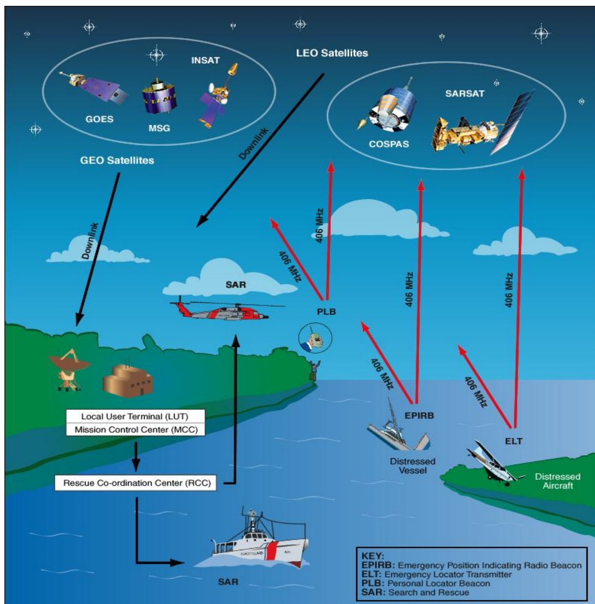
Figure 7: Basic Concept of the Cospas-Sarsat System
