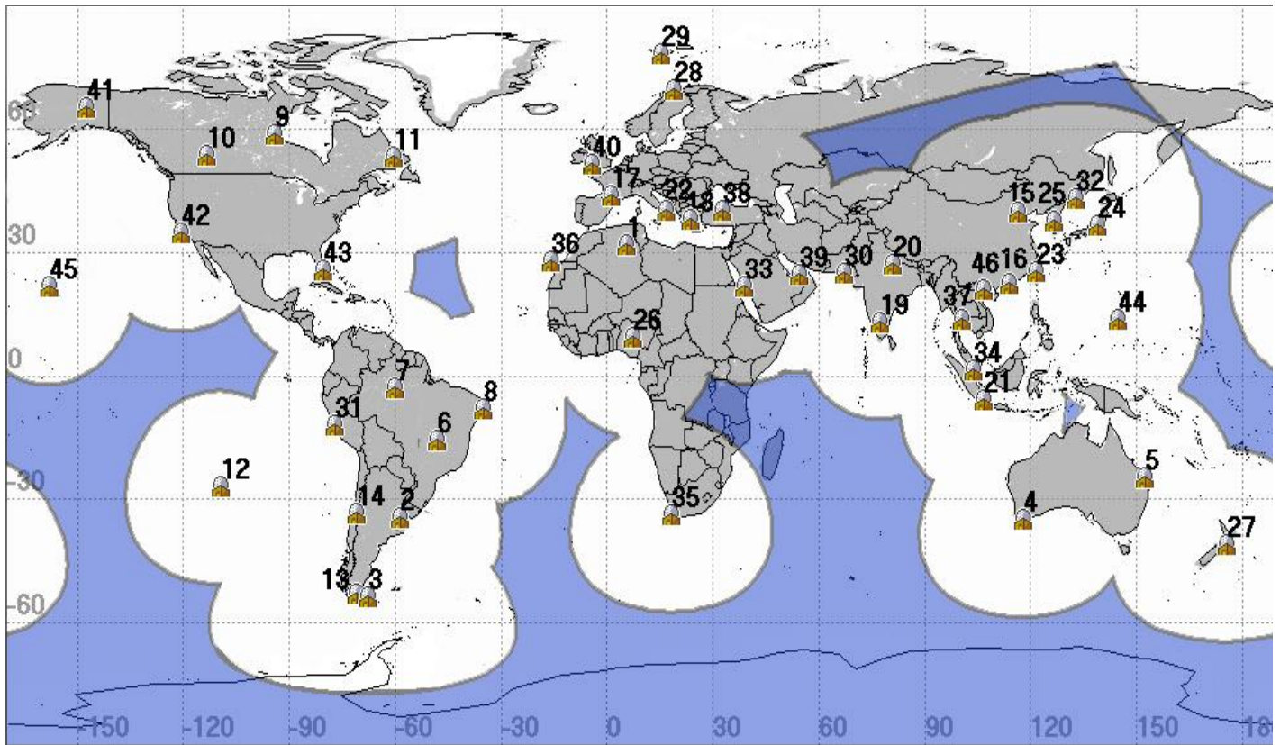
Figure 5: Satellite Visibility Area of Cospas-Sarsat Operational LEOLUTs (15 December 2011)
